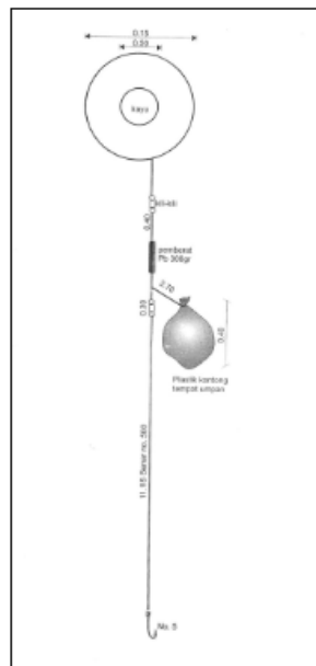
Gambar pancing ulur tuna
