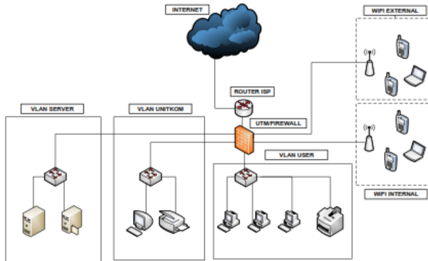
Standar topologi
